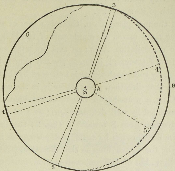
Fig. 2.—The Galactic Cloven Flat Ring (plan).
