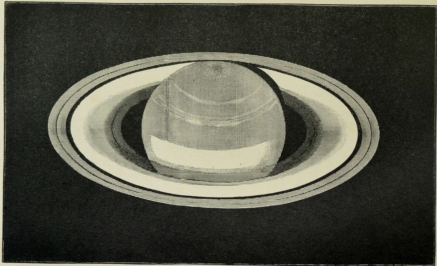
THE PLANET SATURN.
