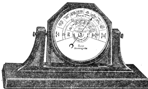
Taylor Stand 'Stormguide.' Walnut finish bakelite easel stand; brass bezel; 4" grained brass dial. No. 13142 Price each $16.00
