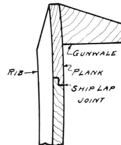
Section "Longitudinal Strip" Construction
