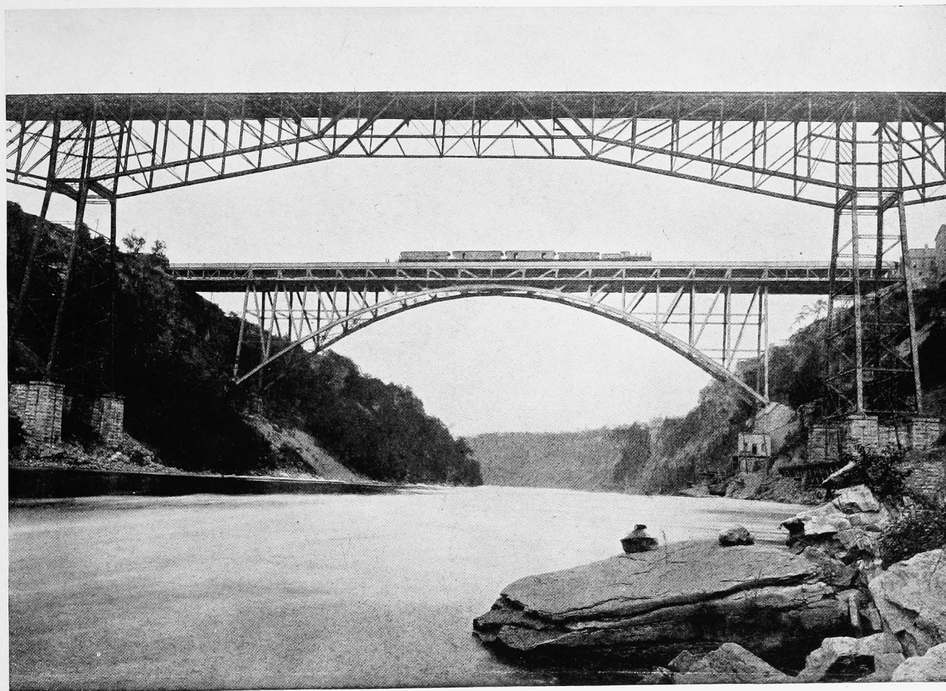
GRAND TRUNK STEEL ARCH AND MICHIGAN CENTRAL CANTILEVER BRIDGES. In the foreground is the double-track cantilever bridge of the Michigan Central Railroad, built 1883. It is 900 feet long. The towers which support it rise 135 feet above their piers. The Steel Arch Bridge beyond was built in 1897, for the use of the Grand Trunk Railway
